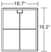
(B) Body - Short Side Qty: 2
